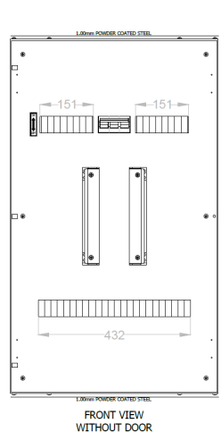
(Technical Drawing )
