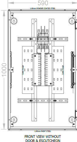
(Technical Drawing )
