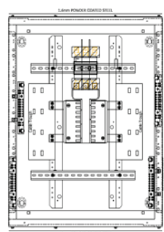
EQUIPMENT LAYOUT DOOR & ESCUTCHEON REMOVED
