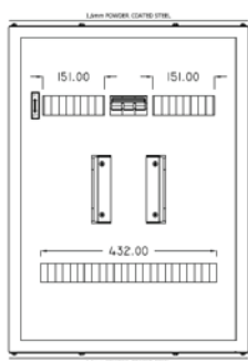
EQUIPMENT LAYOUT DOOR REMOVED
